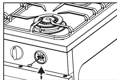
Adjustment location is inside the valve stem
